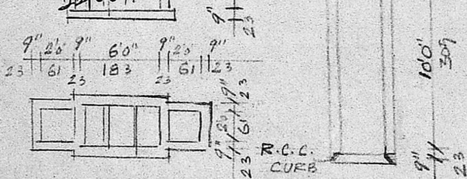
PLAN & SEC OF SEPTIC TANK
